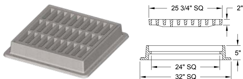
5726 Frame Options (All gray iron)
